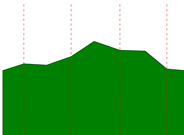
Figure 345: How the Midpoint Displacement Algorithm Works (4/4)
